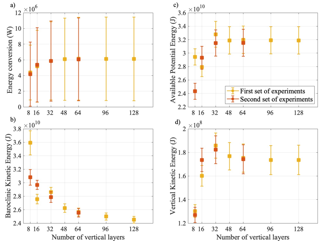
Figure 5. (a) Domain-integrated tidal barotropic-to-baroclinic energy conversion (W), (b) baroclinic (horizontal + vertical) kinetic energy (J), (c) available potential energy (J), and (d) vertical kinetic energy (J) as a function of the number of vertical layers for two grid-discretizations: layers defined using the zero-crossings of u -eigenfunctions (yellow; the first set of experiments), and layers defined by merging layers from the 128-layer simulation (orange; the second set of experiments). All the above were integrated spatially from 0 to 250 km from the center of the ridge, and the error bars are the temporal standard deviation over four tidal cycles.
